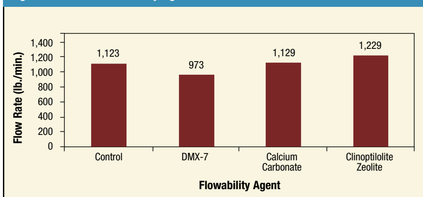
Figure 3. Effect of Flowability Agents on Flow Rate of DDGS Out of a Feed Truck
