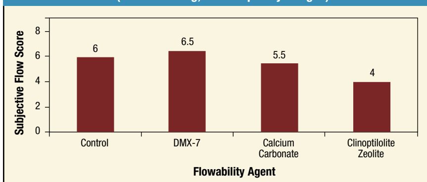
Figure 4. Effect of Flowability Agents on Subjective Flow Score of DDGS Out of a Feed Truck (1=free flowing; 10=completely bridged)
