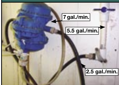
Figure 2. Water Medicator Connected to Waterlines with 1/2-in. Washing Machine Hoses. Note the Estimated Flow Capacities of the Various Components
