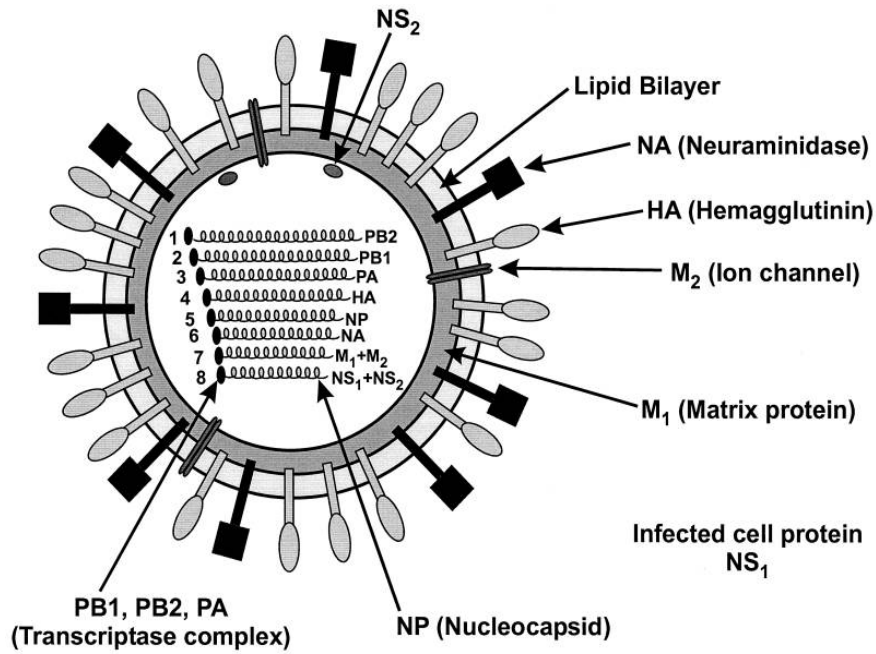
Figure 1. Influenza Virus Structure: Virus and Genome
