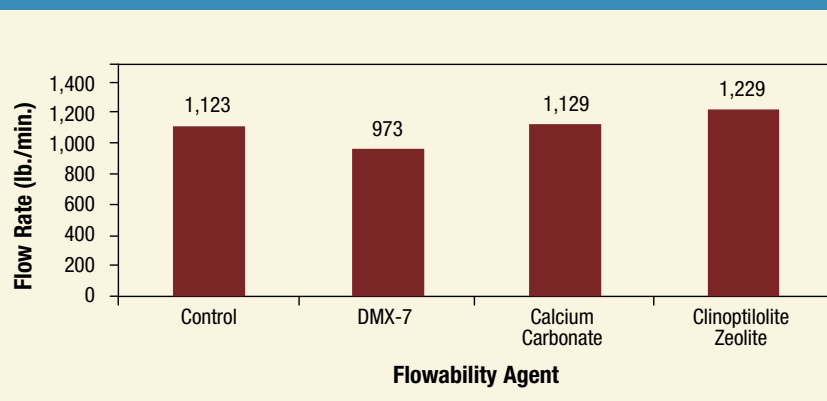
Figure 3. Effect of Flowability Agents on Flow Rate of DDGS Out of a Feed Truck
