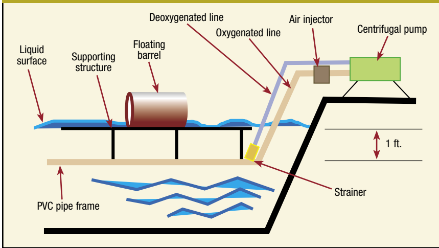
Figure 1. Partial View of the Aeration Apparatus
